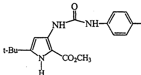
5-tert-Butyl-3-(3-p-tolyl-ureido)-1H-pyrrole-2-carboxylic acid methyl ester
